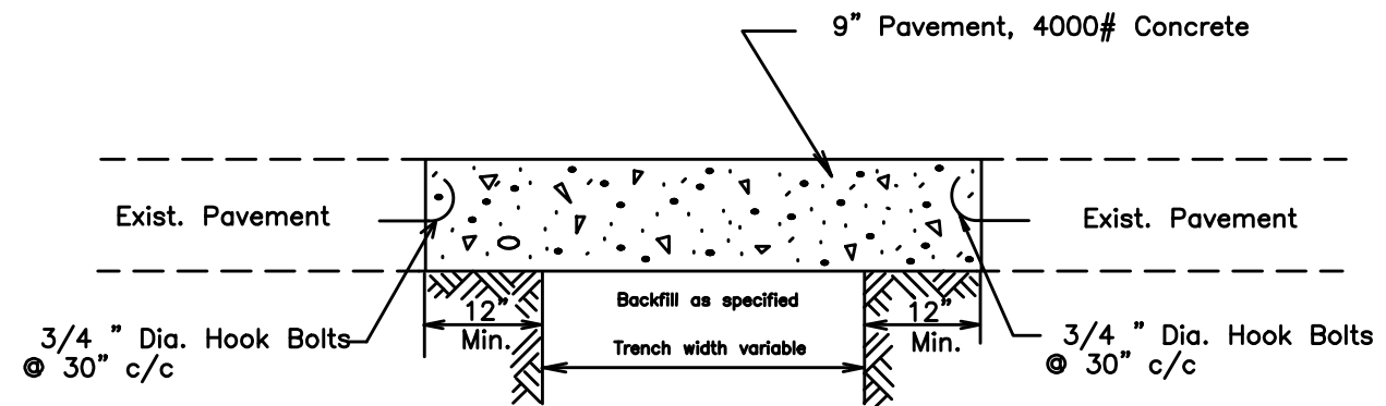
TYPICAL SECTION REPAVING OVER SEWER TRENCH IN PAVEMENTS WITHOUT BASES
