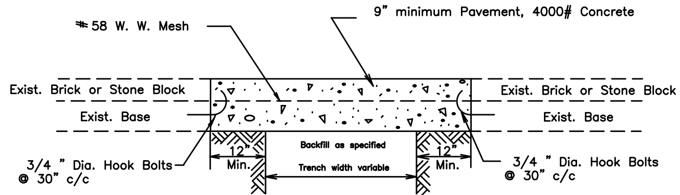
TYPICAL SECTION REPAVING OVER SEWER TRENCH IN BRICK OR STONE BLOCK PAVEMENTS WITH BASES
