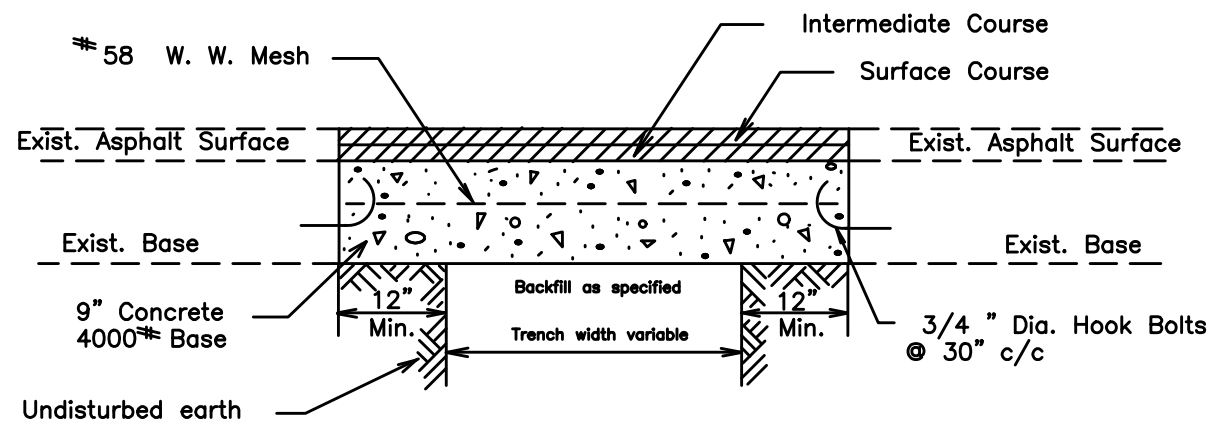
TYPICAL SECTION REPAVING OVER SEWER TRENCH IN ASPHALT PAVEMENT
