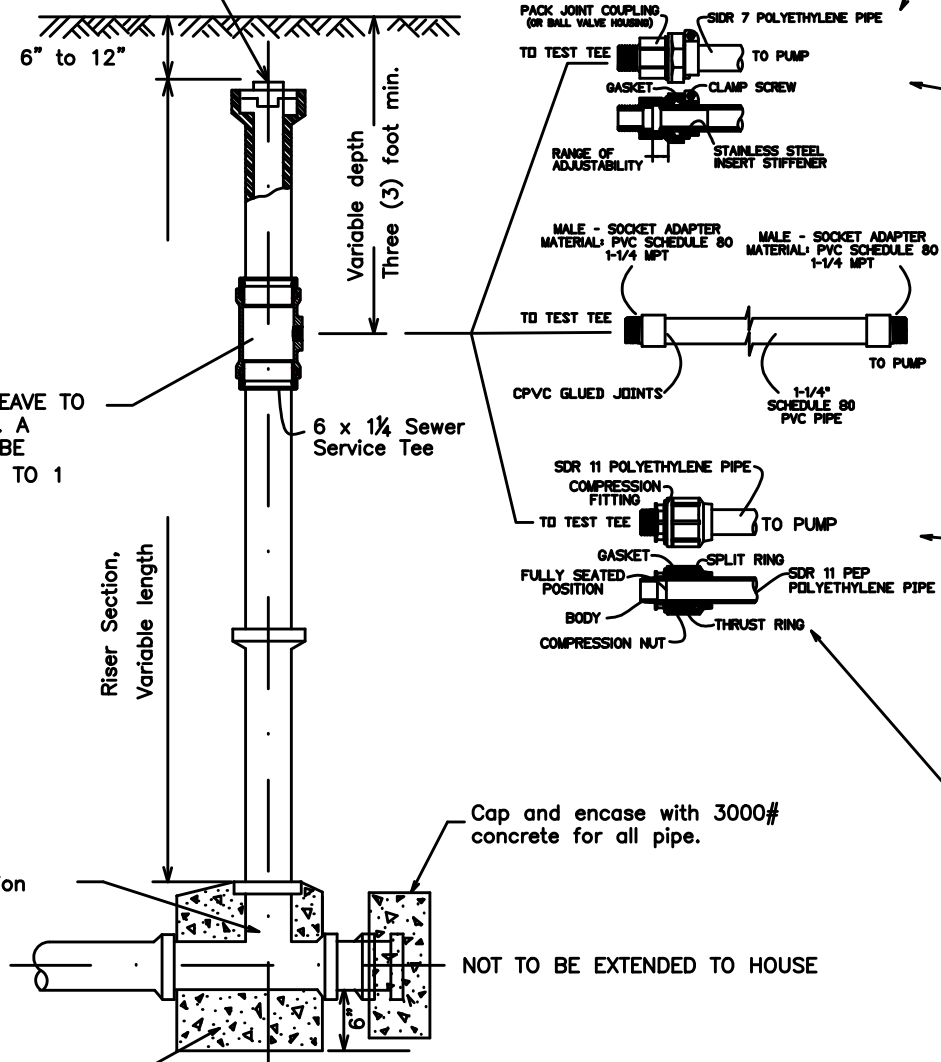
6" X 6" TEST TEE & 6" RISER FOR SANITARY SEWERS.
