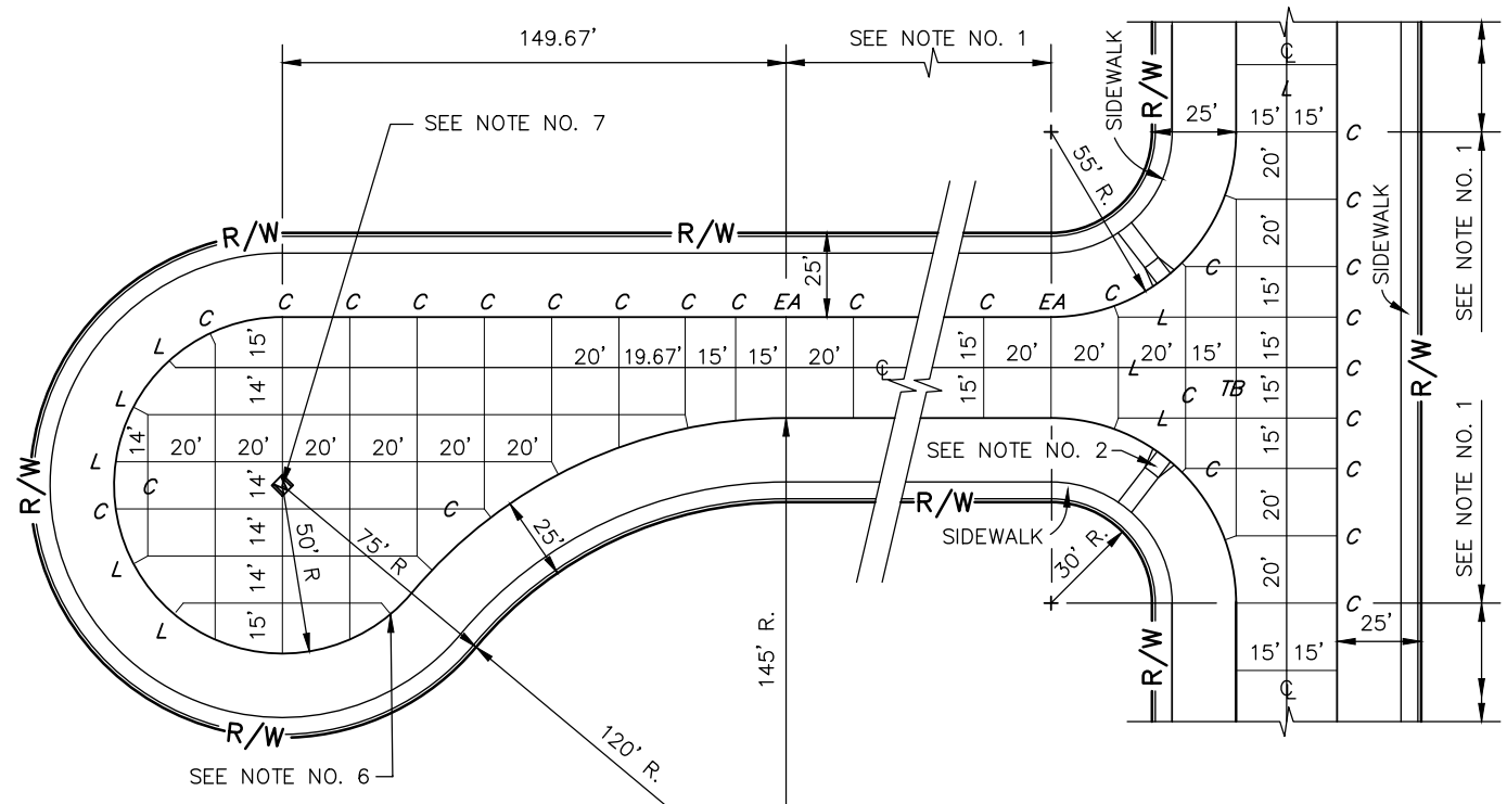
OPTIONAL INTERSECTION AND CUL-DE-SAC DETAIL COMMERCIAL & INDUSTRIAL
