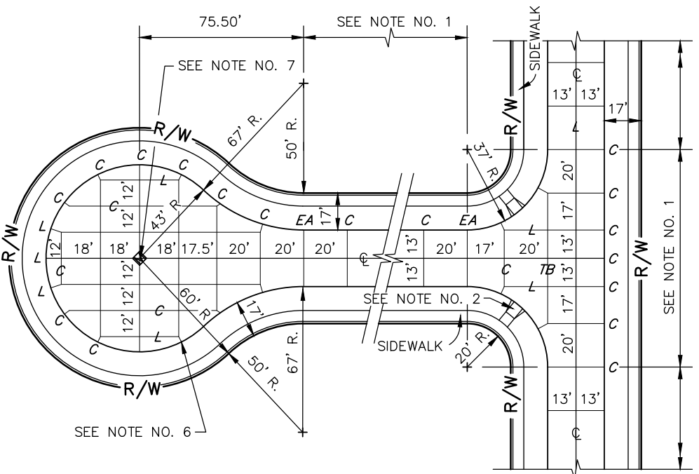
INTERSECTION AND CUL-DE-SAC DETAIL LOCAL RESIDENTIAL
