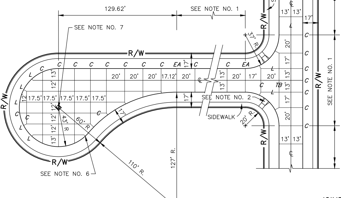
OPTIONAL INTERSECTION AND CUL-DE-SAC DETAIL LOCAL RESIDENTIAL
